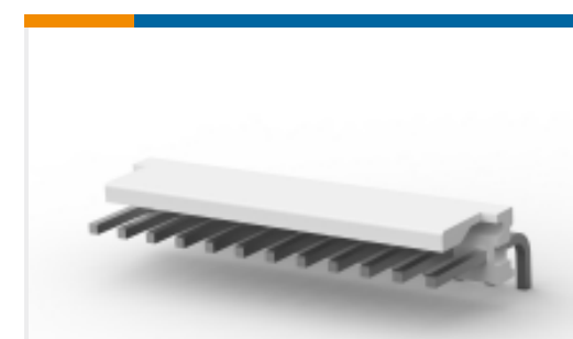
TE Part # 1-640389-2 12P MTA156 HDR ASSY SQ R/A F/L
